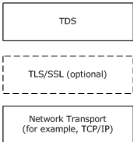
Figure 2: Protocol relationship
